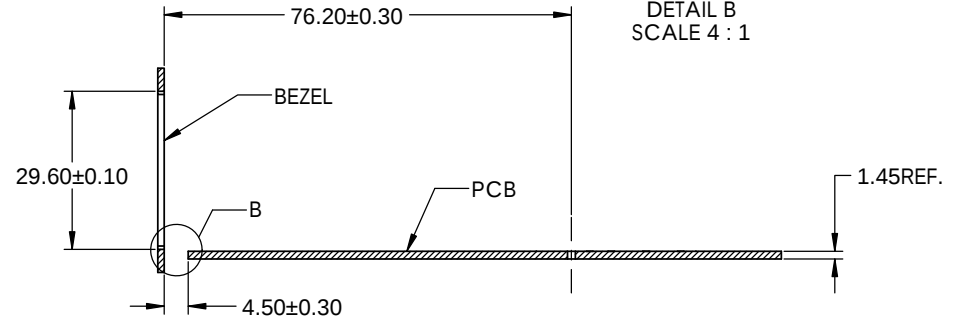
RECOMMENDED BEZEL DESIGN FOR SINGLE SIDE MOUNTING
