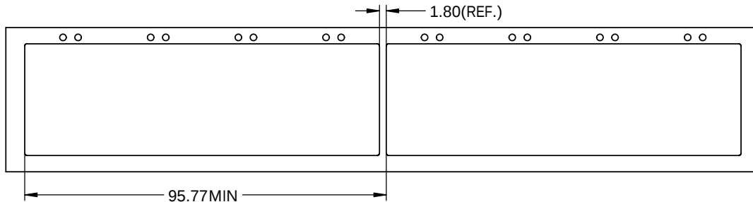
RECOMMENDED BEZEL DESIGN FOR SINGLE SIDE MOUNTING
