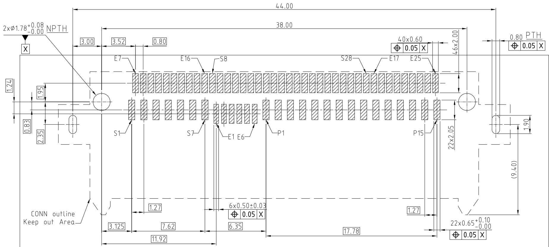
RECOMMENDED PCB LAYOUT(Top View) T=2.0mm GENERAL TOLERANCE \pm 0.05\text{mm}
