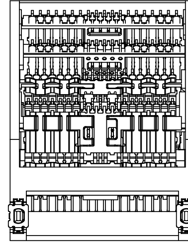
V36-ADZ04-X07100T (WITH SOLDER RINGS FOR BELLY TO BELLY MOUNTING)
